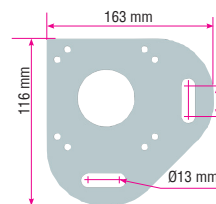
Support de fixation au sol ST4502 Floor fixation support: ST4502
